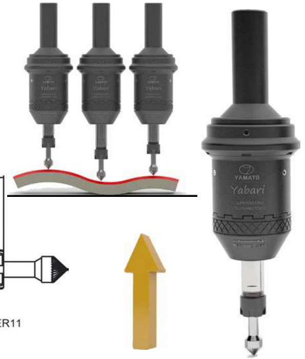
10mm AXIAL DEFLECTION PUSHING
